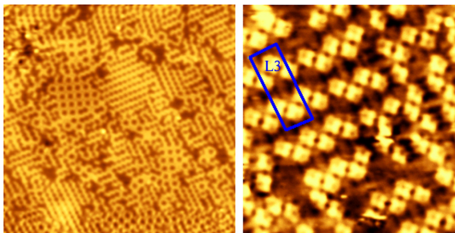
Fig. 3. Filled-state STM images of the surface recorded after a further annealing of the sample for about 20 min still at 260 °C. (a) 50 \times 50 \text{ nm}^2 area ( V = -0.05 \text{ V} , I = 3.7 \text{ nA} ), (b) 10 \times 10 \text{ nm}^2 area ( V = -0.07 \text{ V} , I = 3.4 \text{ nA} ).
